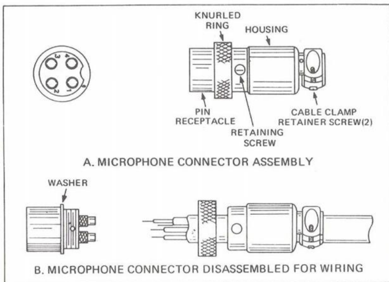
Fig. 4. Microphone plug wiring.
