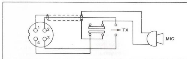
Fig. 3. Your transceiver microphone schematic.
